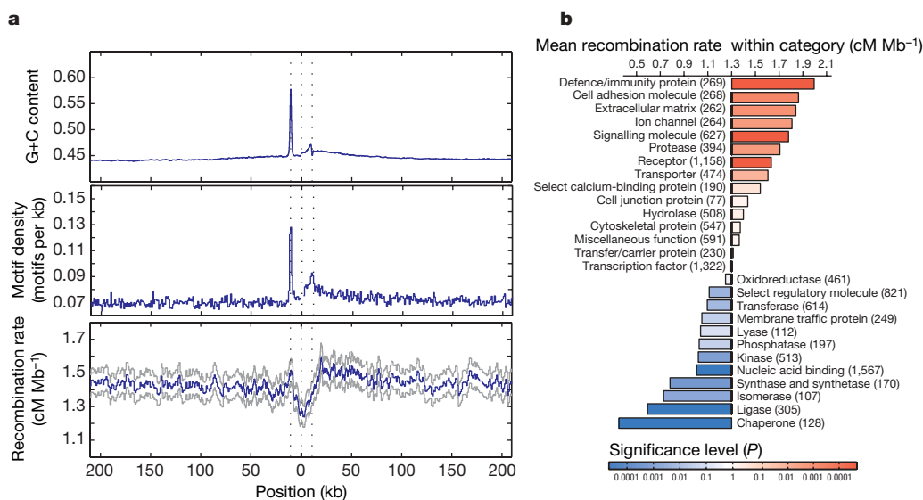
Figure 5 | Recombination rates around genes. a , The recombination rate, density of recombination-hotspot-associated motifs (all motifs with up to 1-bp different from the consensus CCTCCCTNCCAC) and G+C content around genes. The blue line indicates the mean. For the recombination rate, grey lines indicate the quartiles of the distribution. Values were calculated separately 5' from the transcription start site (the first dotted line) and 3' from the transcription end site (third dotted line) and were joined at the median midpoint position of the transcription unit (central dotted line). Note the sharp drop in recombination rate within the transcription unit, the
